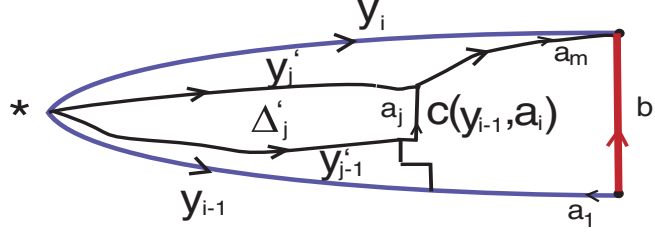
FIGURE 4. Recursive van Kampen diagram
