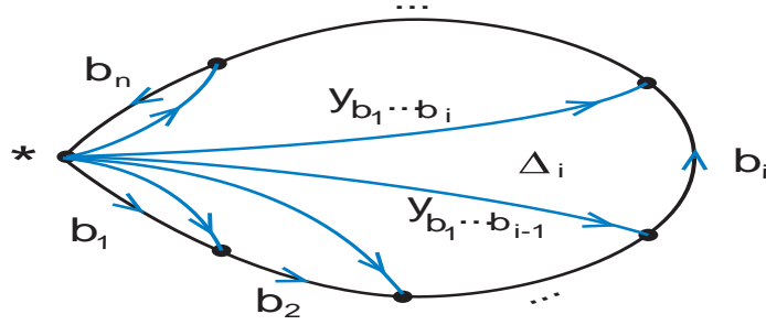
FIGURE 1. Van Kampen diagram built with seashell method
